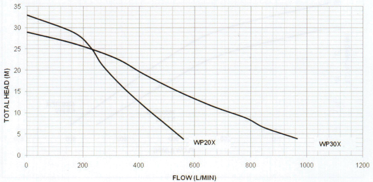
WP30 & 20X PERFORMANCE CURVE
