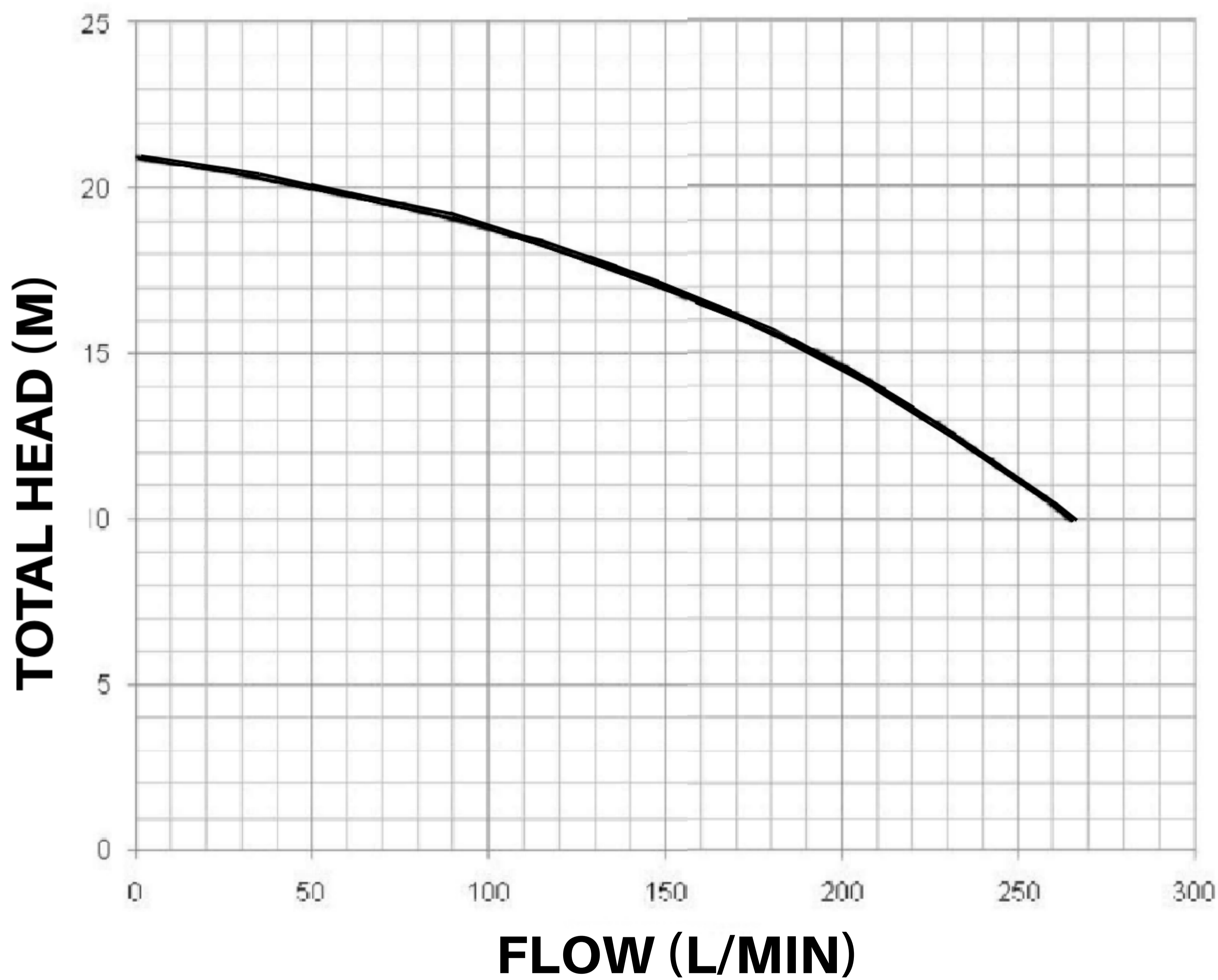
SPA 750 MF PERFORMANCE CURVE
